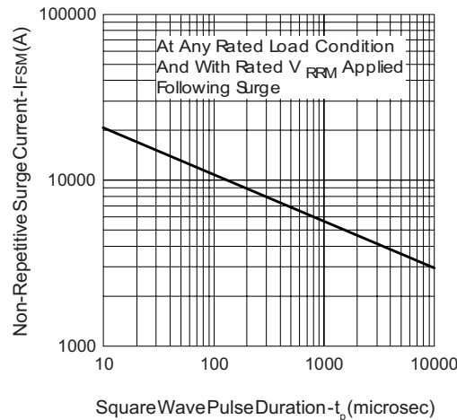
Fig. 7 - Maximum Non-Repitative Surge Current
